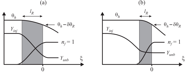
Figure 2: Structure of the reaction layer (RL) for small diffusion (a) and dominant diffusion (b).
