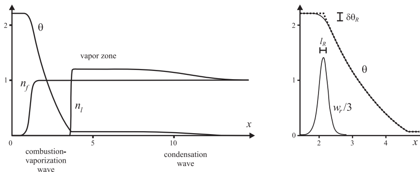
Figure 4: Non-dimensional results of numerical simulation for combustion-vaporization and condensation waves.
