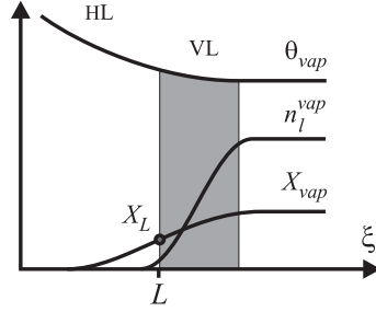
Figure 3: Structure of the vaporization layer (VL).
