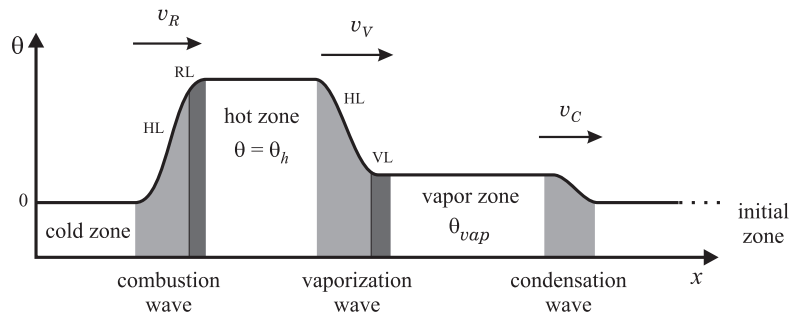
Figure 6: Wave sequence for complete oxygen consumption.
