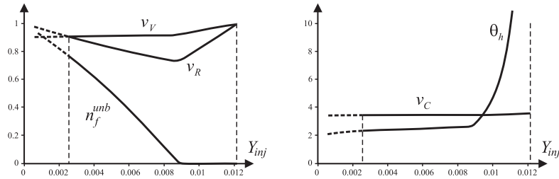
Figure 7: Non-dimensional solution parameters depending on the initial oxygen fraction Y_{inj} .
