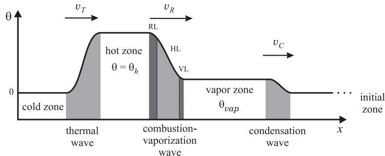
Figure 1: Wave sequence for complete fuel consumption.
