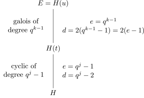
Figure 10: The intermediate field H(t) .
