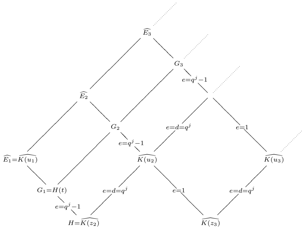
Figure 11: The subfields G_s .
