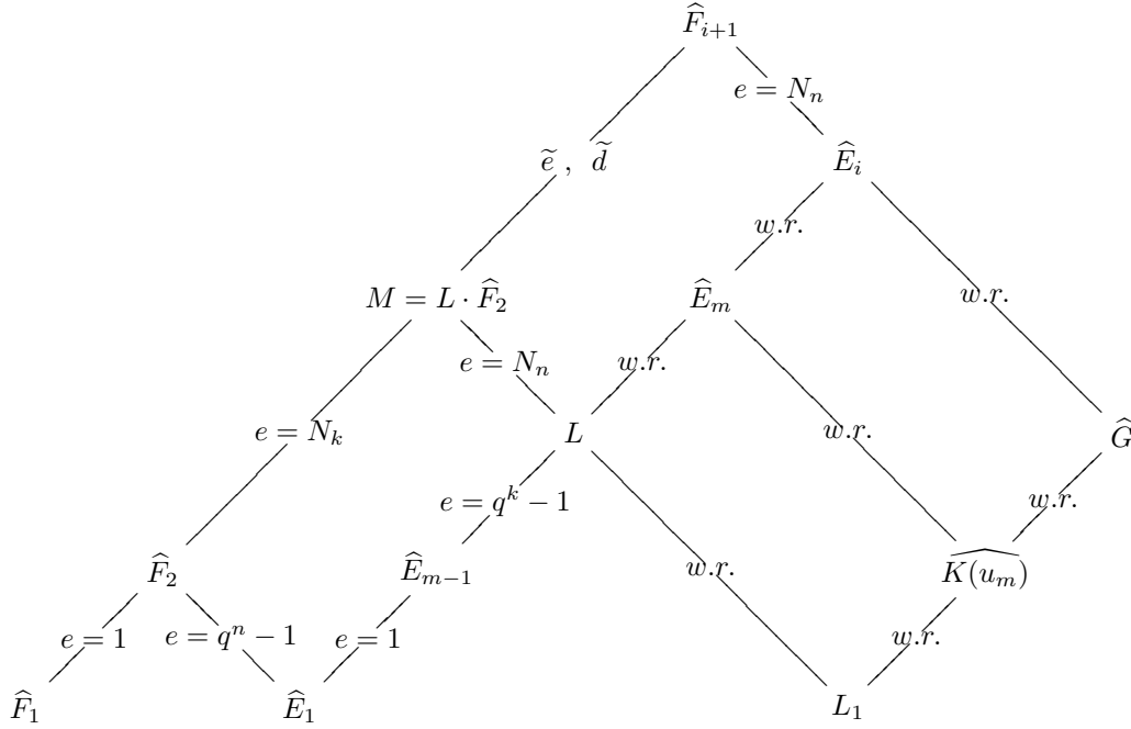
Figure 14: Ramification over \widehat{F}_1 in case m \geq 2 .
