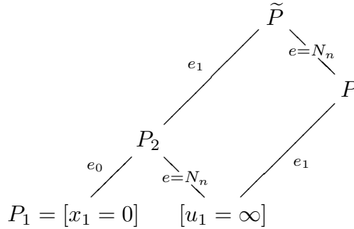
Figure 12: The place extension \widetilde{P}|P_1 in the case m = 1 .
