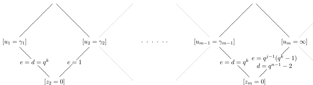
Figure 13: The case m \geq 2 .
