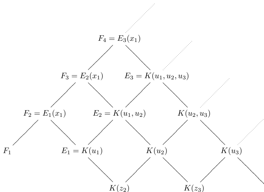
Figure 8: The subtower \mathcal{E} = (E_1 \subseteq E_2 \subseteq \dots) .
