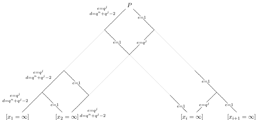
Figure 6: Ramification over [x_1 = \infty] .
