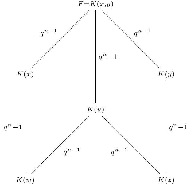
Figure 1: Subextensions of F and their degrees
