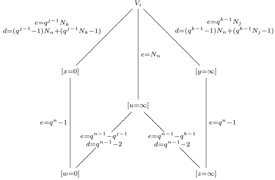
Figure 4: Ramification and different exponents for V_i , 1 \leq i \leq q .
