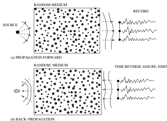
FIGURE 1. Schematic representation of a time reversal experiment in a random medium.
