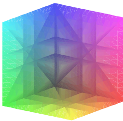
FIGURE 2. Arrangement of 12 hyperplanes on \mathbb{P}^3 associated to D_4
